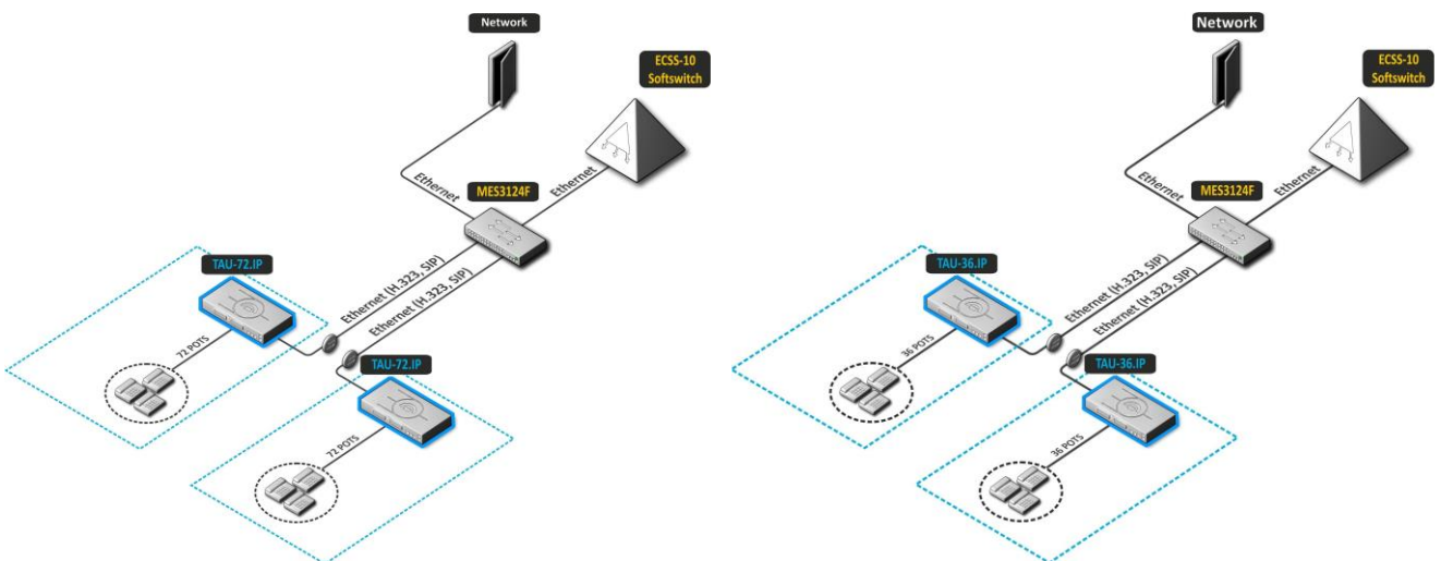
Fig 2 - TAU-72.IP/TAU-36.IP distributed mini-PABX
