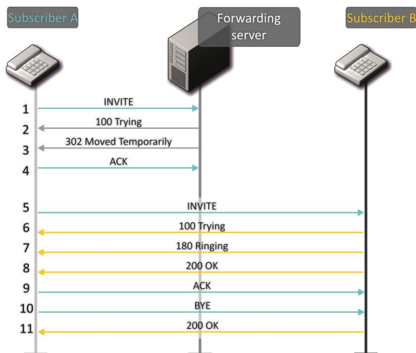
Fig. 17—Call algorithm involving forwarding server
