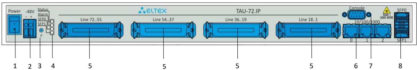
Fig. 4b - TAU-72.IP v3.0 front panel appearance
