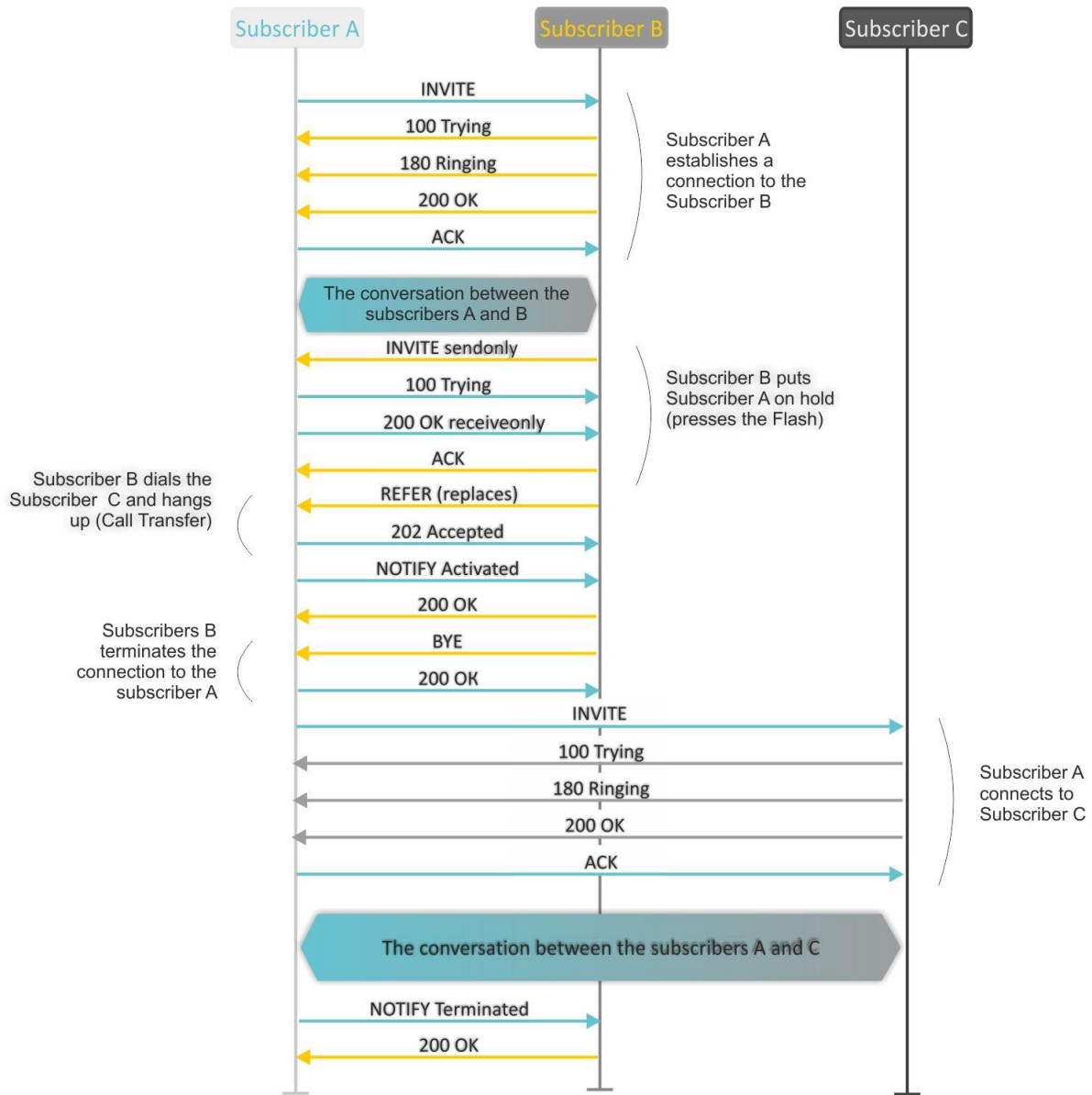
Fig. 11—Algorithm of 'Unattended call transfer' service performed by Subscriber B via SIP protocol
