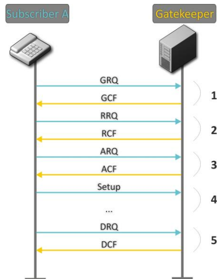
Fig. 19—Gatekeeper call algorithm
