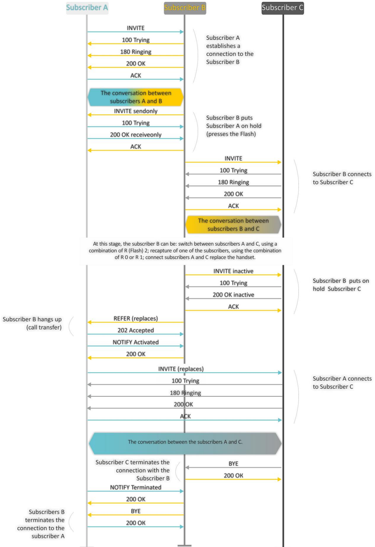
Fig. 10—Algorithm of 'Attended call transfer' service performed by Subscriber B via SIP protocol
