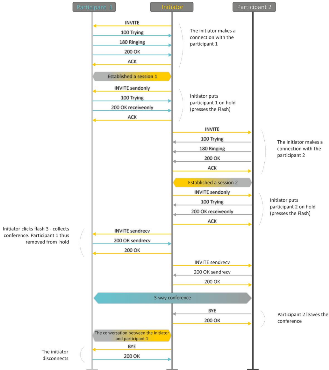
Fig. 12—Algorithm of '3-way conference' service performed locally on the device via SIP protocol
