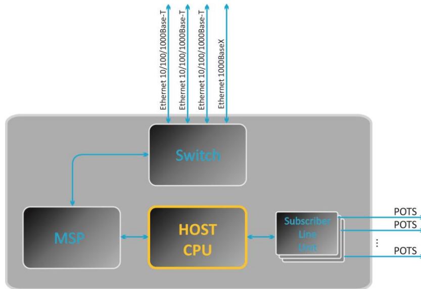
Figure 3a - TAU-72.IP functional diagram
