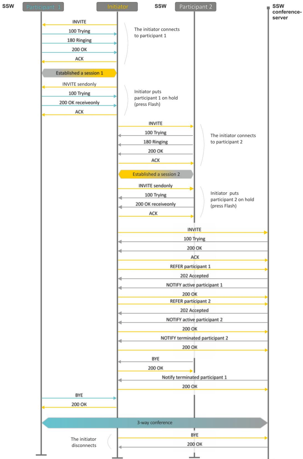
Fig. 13—Algorithm of '3-way conference' service performed at the conference server via SIP protocol (REFER to focus)
