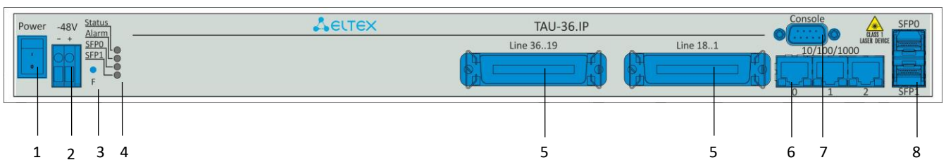
Fig. 4e - TAU-36.IP with DC power supply front panel appearance
