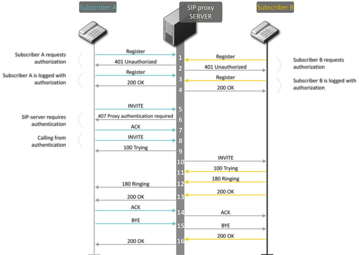
Fig. 16—Call algorithm involving SIP proxy server
