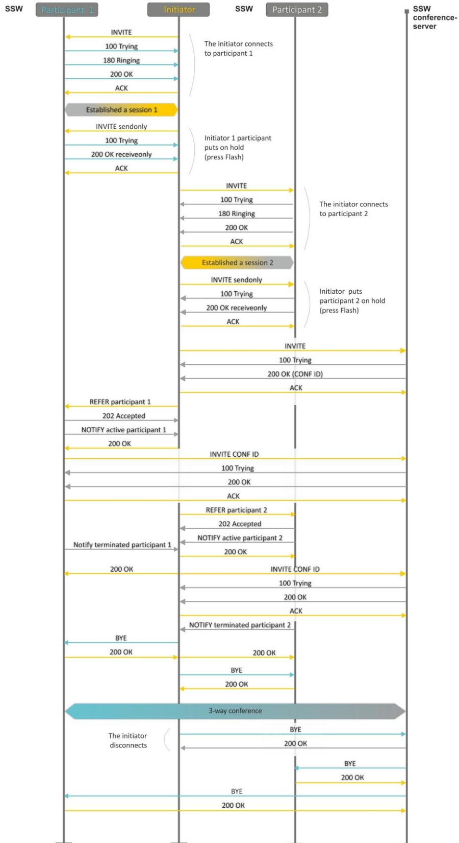
Fig. 14—Algorithm of '3-way conference' service performed at the conference server via SIP protocol (REFER to user)
