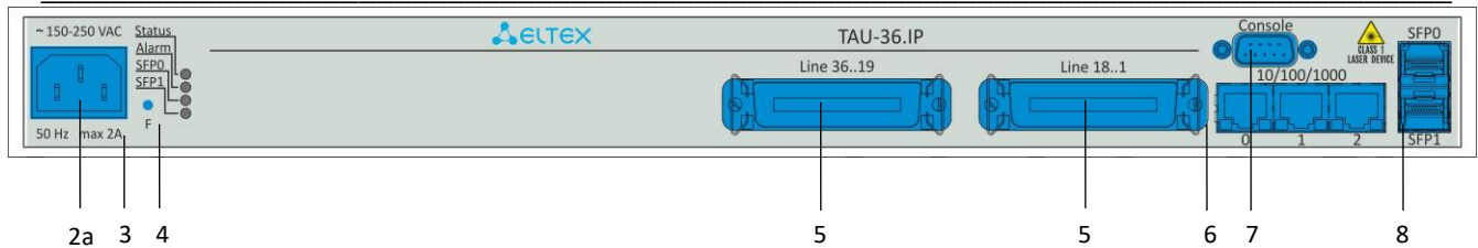
Fig. 4f - TAU-36.IP with AC power supply front panel appearance
