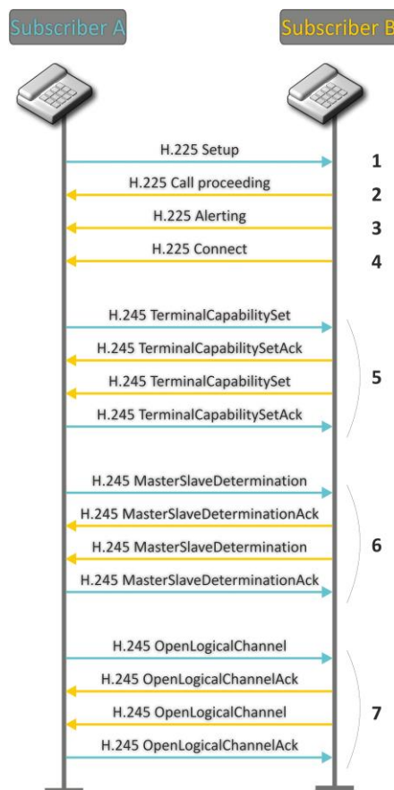
Fig. 18—H.323 call algorithm
