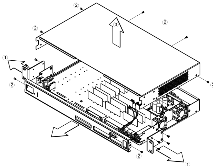
Fig. 7 - TAU-72.IP/TAU-36.IP case opening order
