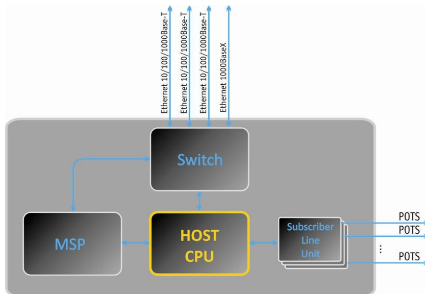
Figure 3b - TAU-36.IP functional diagram
