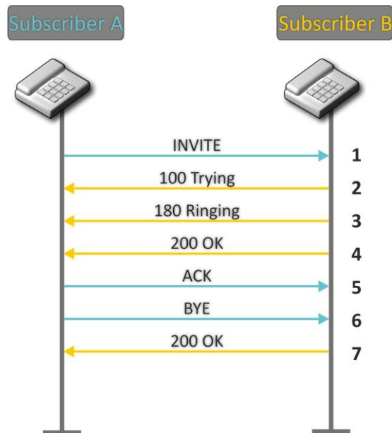
Fig. 15—SIP call algorithm
