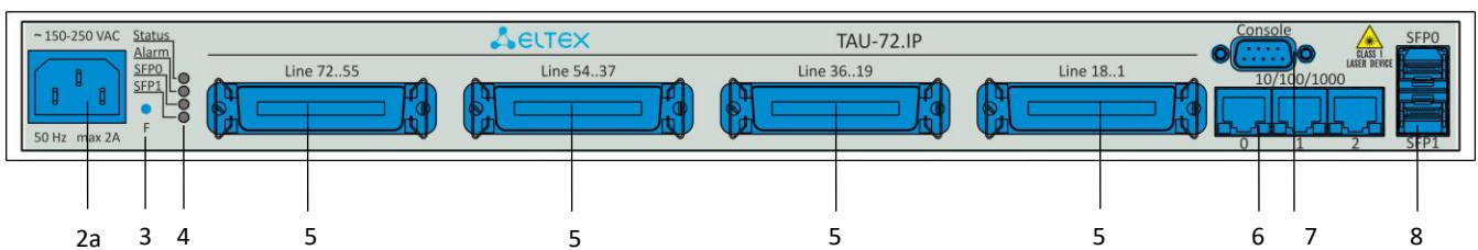
Fig. 4d - TAU-72.IP v4.0 and rev.B with AC power supply front panel appearance
