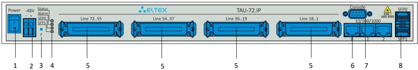
Fig. 4c - TAU-72.IP v4.0 and rev.B with DC power supply front panel appearance
